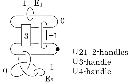
FIGURE 12. E(2)\#2\overline{\mathbf{CP}^2}
