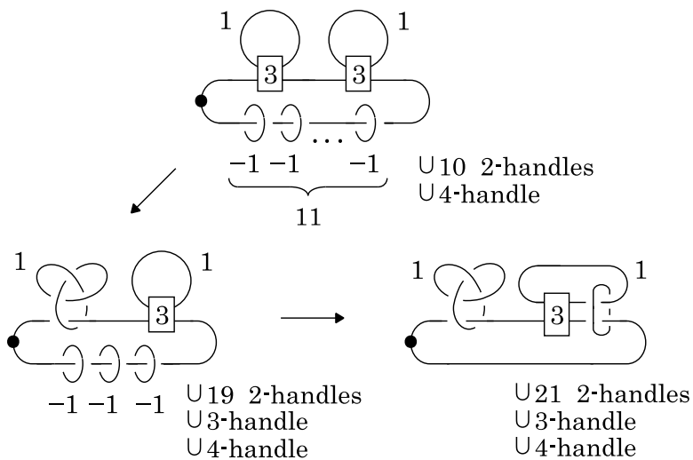
FIGURE 17. handle moves of E(2)
