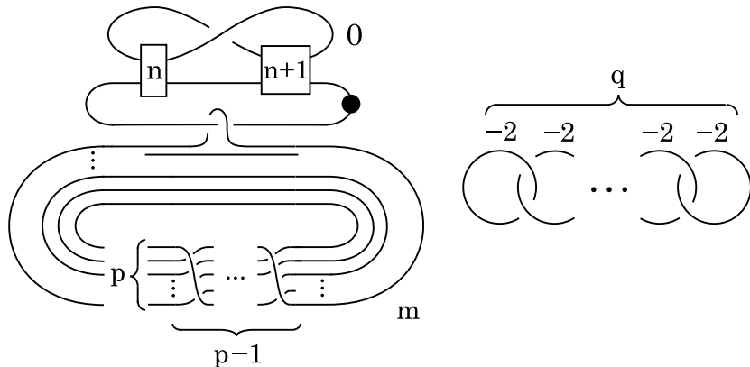
FIGURE 2. C_1(m, n, p, q)
