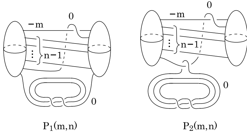
FIGURE 11. P_1(m, n) and P_2(m, n)
