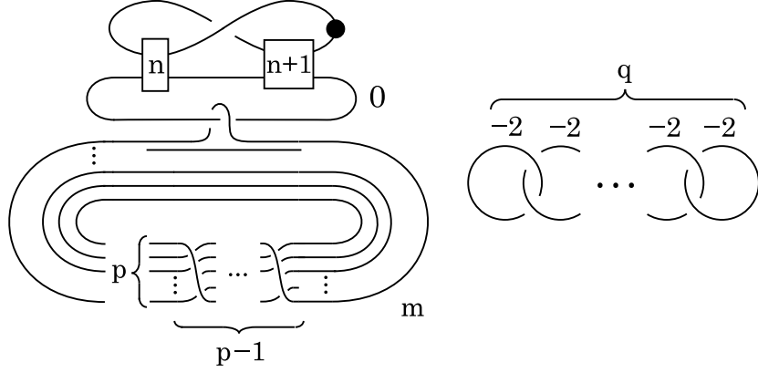
FIGURE 3. C_2(m, n, p, q)
