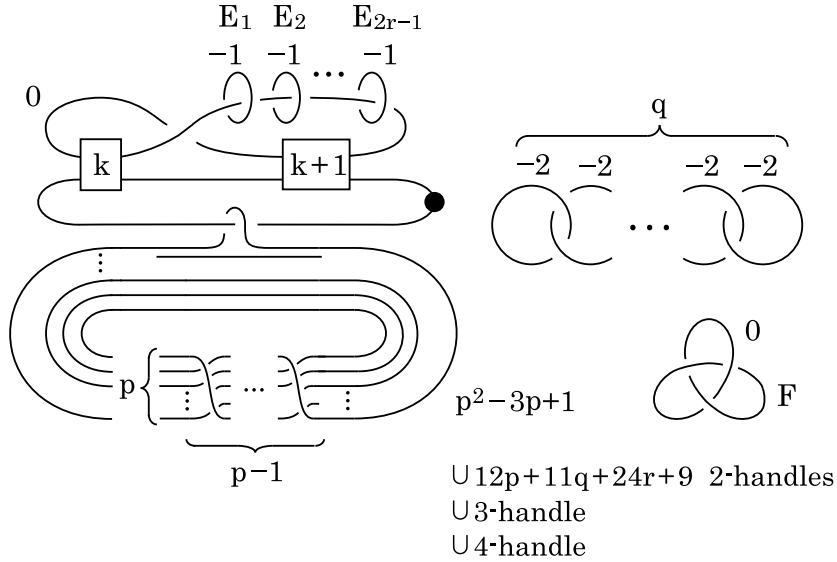
FIGURE 9. E(p+q+2r+1)\#(2r-1)\overline{\mathbf{CP}^2} ( k = 3r-2, 3r-1, 3r )
