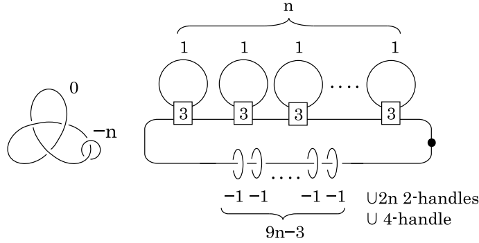
FIGURE 7. E(n)
