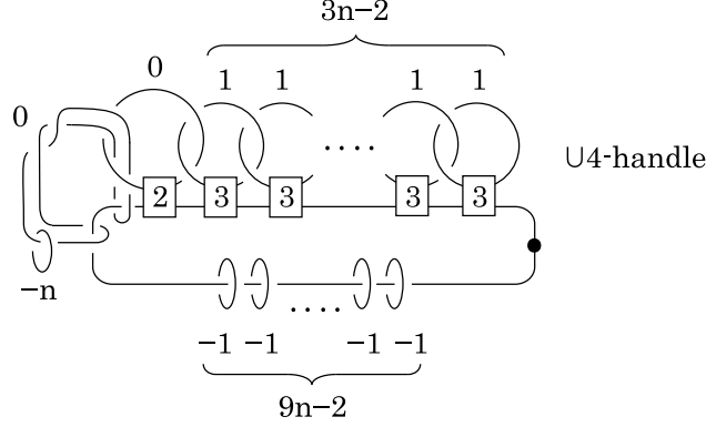
FIGURE 6. E(n)
